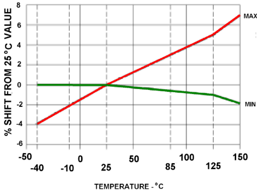
SENSITIVITY SHIFT vs TEMPERATURE
